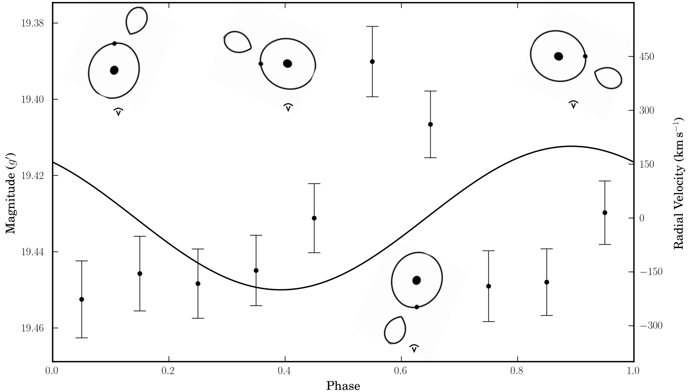
FIG. 10.— Phase-binned light curve taken on 2011 Mar 04 using the P60. 87 60 s exposures were binned into 10 bins with a zero phase of HJD = 2455624.81212, the start of the phase-resolve spectroscopy, and the spectroscopically derived period of 26.77 m. Overplotted is the S-wave found in §4.2. The rough orientation of the binary is shown with drawings at the four extreme points of the orbit, along with the position of the observer.
