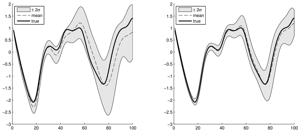
Figure 2: Mackey-Glass 100-step ahead prediction benchmark. Left: standard GP using 200 randomly drawn training inputs. Right: FITC with 40 pseudo-inputs.
