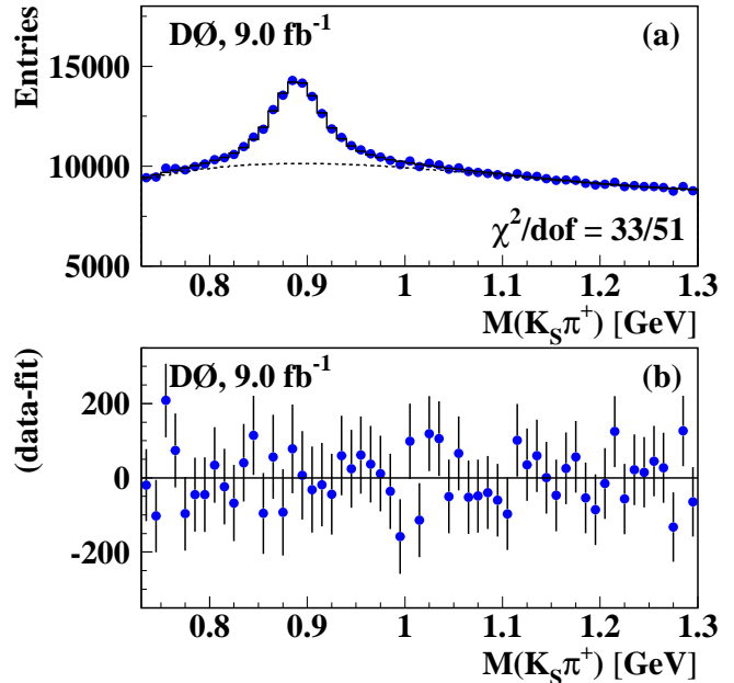
FIG. 3: (color online). (a) The K_S^0\pi^+ invariant mass distribution for K^{*+} candidates in the inclusive muon sample. The K_S^0 candidate is required to have 480 < M(\pi^+\pi^-) < 515 MeV and 4.2 < p_T(K_S^0) < 5.6 GeV. The solid line represents the result of the fit to the K^{*+} content, and the dashed line shows the background contribution. (b) Difference between data and the result of the fit.
