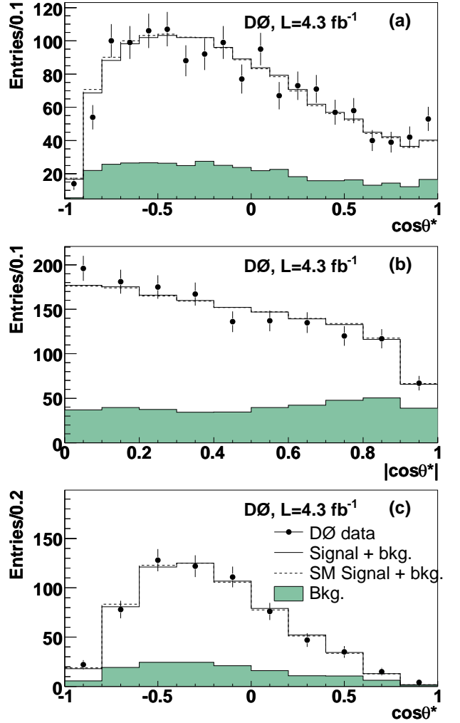
FIG. 11: (Color online) Comparison of the \cos \theta^* distribution in Run IIb data and the global best-fit model (solid line) and the SM (dashed line) for (a) leptonic W boson decays in \ell +jets events, (b) hadronic W boson decays in \ell +jets events, and (c) dilepton events.
