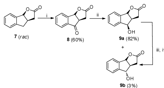
Scheme 1 Reagents and conditions: (i) FeCl 3 (2 mol%), aq TBHP (70%, 3 equiv) pyridine, 82 °C, 24 h, (ii) NaBH 4 , CeCl 3 ·7H 2 O, EtOH, (iii) PPh 3 , PhCO 2 H, EtO 2 CN=NCO 2 Et, toluene, (iv) K 2 CO 3 , MeOH.
