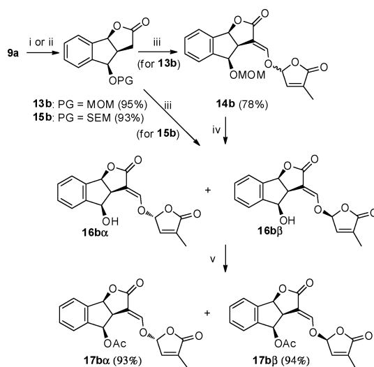
Scheme 3 Reagents and conditions: (i) MOM chloride, DIPEA, CH 2 Cl 2 , rt, 16 h, (ii) DIPEA, SEMCl, CH 2 Cl 2 , 22 h, (iii) HCO 2 Me, t -BuOK, THF, then butenolide 10 , DME, workup with 1 M HCl (iv) ZnBr 2 , CH 2 Cl 2 , 25 °C, (v) Ac 2 O, pyridine, CH 2 Cl 2 .
