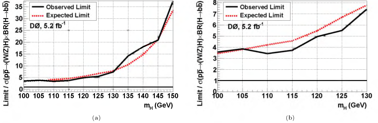
FIG. 9: (a) Ratio of the observed (solid black) and expected (dotted red) exclusion limits to the SM production cross section multiplied by branching fraction for H \rightarrow bb , as a function of m_H , (b) The same zoomed in the low mass region.
