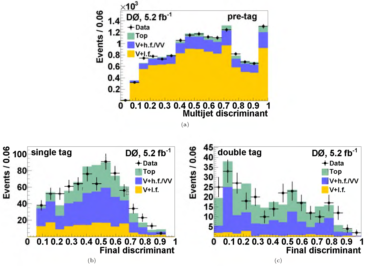
FIG. 8: Discriminants in the EW-control sample: (a) Multijet discriminant, (b) Final single tag discriminant in the single tag sample, (c) Final double tag discriminant in the double tag sample.
