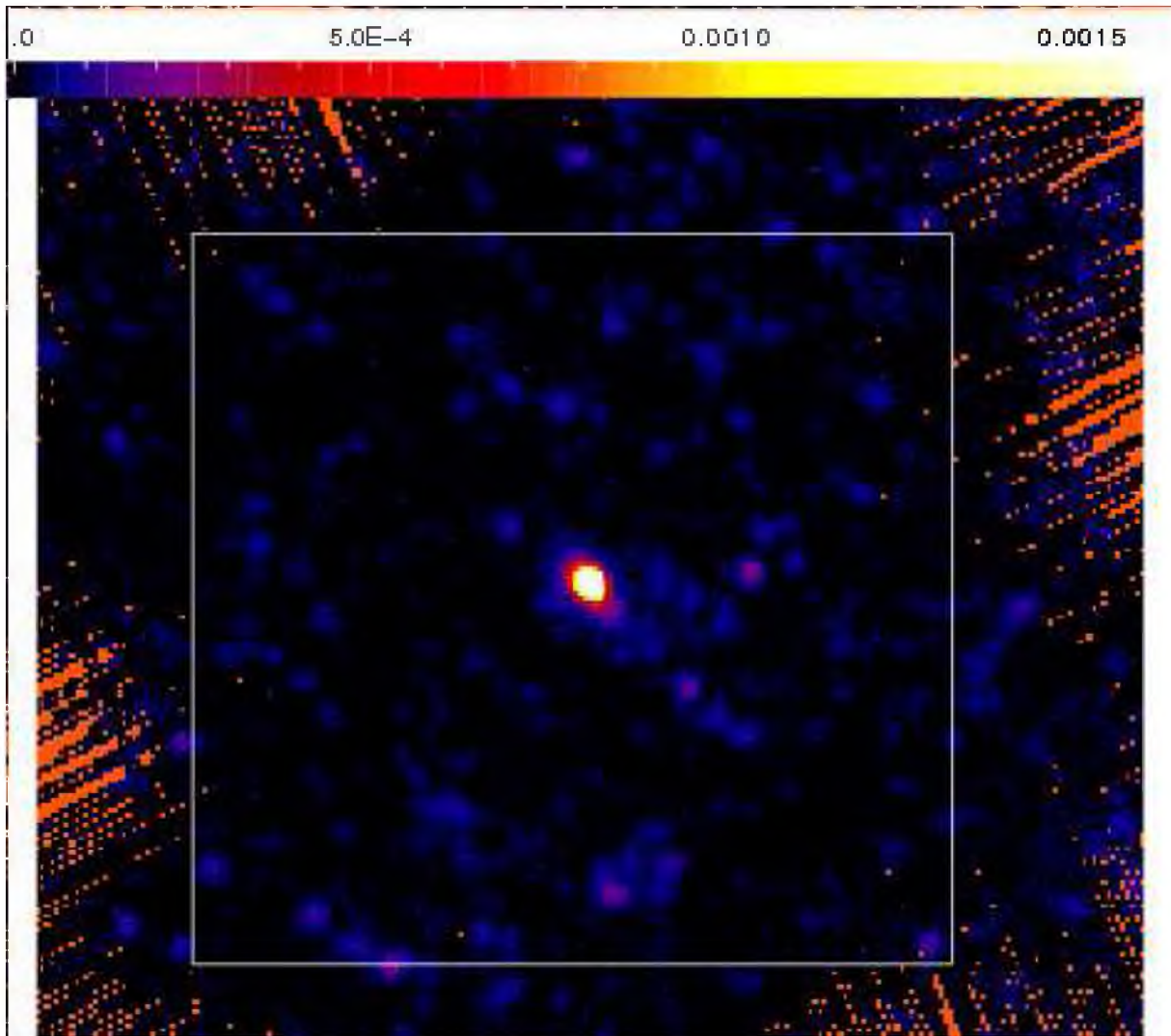
Fig. A.2. The 250 \mu\text{m} SPIRE map around the \beta Pic disk. The 10x10' region delimited by the white square shows more than 50 background sources comparable to the cold blob seen in the southwest of the disk.
