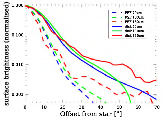
Fig. 4. Normalised surface brightness profiles along the disk in NE direction in the three PACS filters. The profiles were convolved with a Gaussian to match the spatial resolution of the 160 \mu\text{m} image. The same convolved profiles are shown for the PSF maps.
