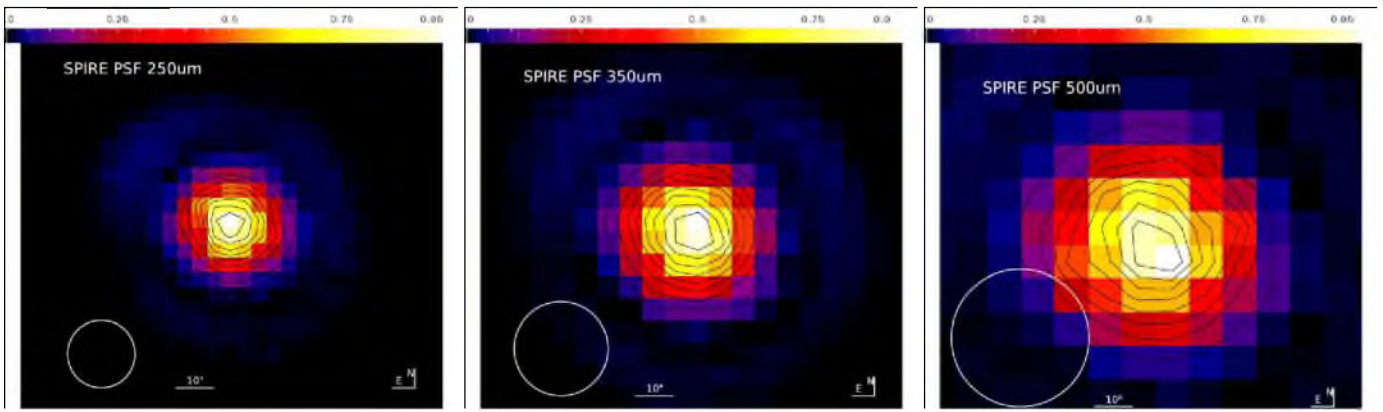
Fig. A.6. The 250, 350 and 500 \mu\text{m} SPIRE PSFs, rotated to match the position angle at the time of the \beta Pic observations. The PSF images are scaled linearly, contour lines are in steps of 10% of the peak flux. The white circle shows the beam FWHM.
