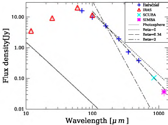
Fig. 5. The infrared to mm SED of \beta Pic. The PACS (70 – 160 \mu\text{m} ), and the SPIRE (250 – 500 \mu\text{m} ) fluxes were integrated over a 60'' radius aperture. IRAS flux densities are from the IRAS Point Source Catalog. The 850 \mu\text{m} SCUBA datum (Holland et al. 1998) and the 1200 \mu\text{m} SIMBA datum (Liseau et al. 2003) are integrated over a 40'' radius aperture. Overplotted is a Rayleigh-Jeans extrapolation of the 160 \mu\text{m} flux density with a spectral index \beta=0 and \beta=2 , and the best fit to the 160–1200 \mu\text{m} data ( \beta=0.34 ). The stellar photosphere is a Kurucz model for T_{\text{eff}}=9000\text{K} ; \log(g)=3.9 scaled to the 2MASS photometry K_s=3.52 .
