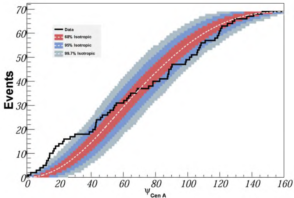
Fig. 9.— Cumulative number of events with E \geq 55 EeV as a function of angular distance from the direction of Cen A. The bands correspond to the 68%, 95%, and 99.7% dispersion expected for an isotropic flux.
