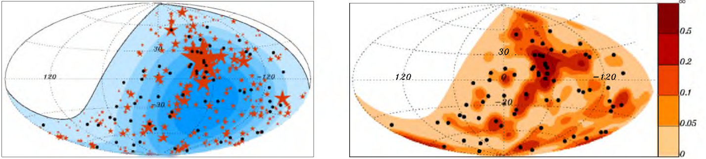
Fig. 4.— Left: Sky map in galactic coordinates with the AGNs of the 58-month Swift-BAT catalog plotted as red stars with area proportional to the assigned weight. The solid line represents the field of view of the Southern Observatory. Coloured bands have equal integrated exposure, and darker background colours indicate larger relative exposure. Right: density map derived from the map to the left, smoothed with an angular scale \sigma = 5^\circ . The 69 arrival directions of CRs with energy E \geq 55 EeV detected with the Pierre Auger Observatory are plotted as black dots.
