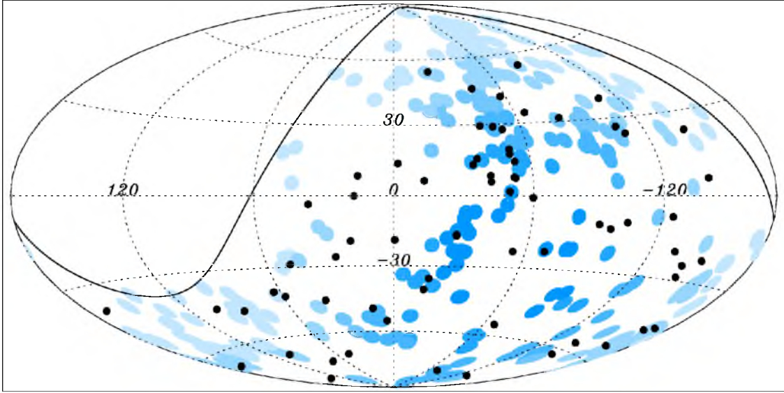
Fig. 1.— The 69 arrival directions of CRs with energy E \geq 55 EeV detected by the Pierre Auger Observatory up to 31 December 2009 are plotted as black dots in an Aitoff-Hammer projection of the sky in galactic coordinates. The solid line represents the field of view of the Southern Observatory for zenith angles smaller than 60^\circ . Blue circles of radius 3.1^\circ are centred at the positions of the 318 AGNs in the VCV catalog that lie within 75 Mpc and that are within the field of view of the Observatory. Darker blue indicates larger relative exposure. The exposure-weighted fraction of the sky covered by the blue circles is 21%.
