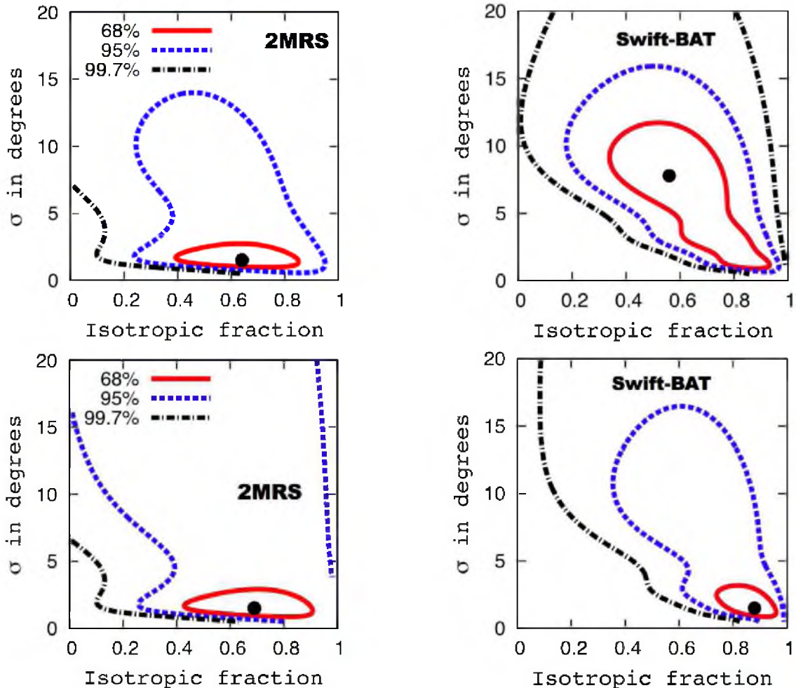
Fig. 6.— Confidence intervals for the parameters (\sigma, f_{\text{iso}}) derived from the likelihood function using the arrival directions of CRs with E \geq 55 EeV for the two models considered: 2MRS galaxies (left) and Swift-BAT AGNs (right). The pair of parameters that maximise the likelihood is indicated by a black dot. The plots in the top panels use all data. The plots in the bottom panels exclude data collected during period I in Table 1, that were used to choose the energy threshold that maximized the correlation with VCV objects in that period. In the case of 2MRS galactic latitudes (both of galaxies and CRs) are restricted to |b| > 10^\circ .
