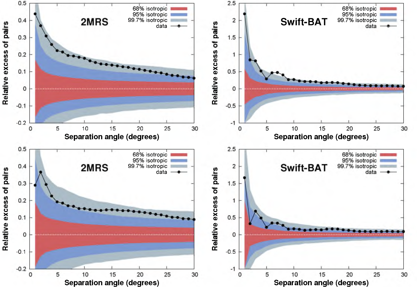
Fig. 3.— Cross-correlation between the arrival directions of CRs measured by the Pierre Auger Observatory with E \geq 55 EeV and positions of 2MRS galaxies (left) and Swift-BAT AGN (right) that lie within 200 Mpc. In the case of 2MRS galactic latitudes (both of galaxies and CRs) are restricted to |b| > 10^\circ . The plots in the top panels use all CRs with E \geq 55 EeV. The plots in the bottom panels exclude data collected during period I in Table 1, that were used to choose the energy threshold and redshift that maximized the correlation with VCV objects in that period. The bands correspond to the 68%, 95% and 99.7% dispersion expected for an isotropic flux.
