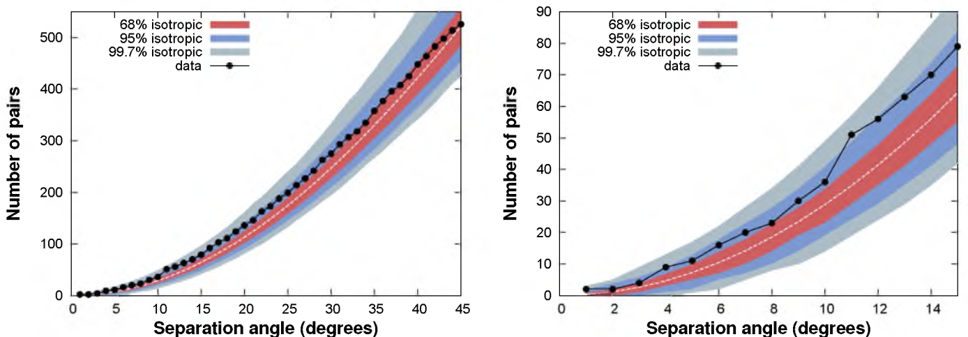
Fig. 8.— Cumulative autocorrelation function for the set of 69 events with E \geq 55 EeV (black dots). The bands correspond to the 68%, 95% and 99.7% dispersion expected for an isotropic flux. The plot in the right panel is an enlarged version of the left plot restricted to angles less than 15^\circ .
