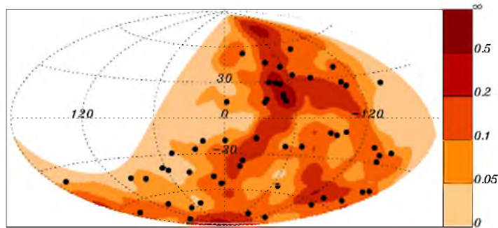
Fig. 5.— Cosmic ray density map for the flux-weighted 2MRS galaxies, smoothed with an angular scale \sigma = 5^\circ . The black dots are the arrival directions of the CRs with energy E \geq 55 EeV detected with the Pierre Auger Observatory. Galactic latitudes are restricted to |b| > 10^\circ , both for galaxies and CR events.
