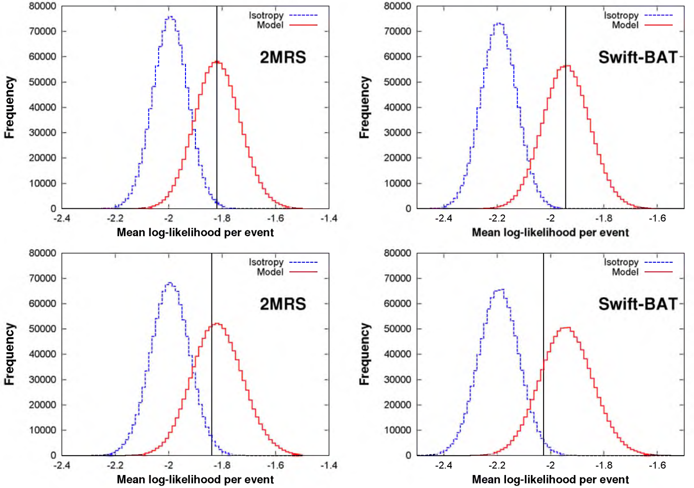
Fig. 7.— Distributions of mean log-likelihood per event for isotropic arrival directions (blue, dashed line histograms) and for the model predictions (red, solid line histograms). The parameters for the models based on the 2MRS galaxies (left) and Swift-BAT AGNs (right) are those that maximize the likelihood with all data, namely (1.5^\circ, 0.64) for 2MRS and (7.8^\circ, 0.56) for Swift-BAT. The value of the log-likelihood for the data is indicated by a black vertical line. The plots in the top panels use all data, and those in the bottom panels exclude data collected during period I.
