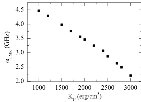
FIG. 7. Ferromagnetic resonance frequency \omega_{\text{FMR}} as a function of the uniaxial anisotropy constant K_U calculated from the FMR formula (Ref. 20). The external field was constant at 0.4 kG applied along the [100] crystallographic direction.
