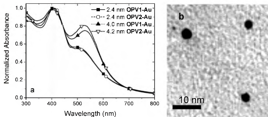
Figure 1. (a) Normalized UV–vis absorption spectra of OPV1–Au ( d_{\text{Au}} = 2.4 and 4.0 nm) and OPV2–Au nanoparticles ( d_{\text{Au}} = 2.4 and 4.2 nm) in toluene. (b) TEM image of the OPV–Au particles cast from dilute toluene solution with d_{\text{Au}} = 4 nm.
