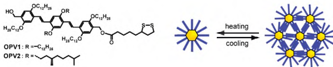
Chart 1. Chemical structure of two oligo( p -phenylene vinylene) (OPV) derivatives ( OPV1 and OPV2 ), both bearing hydroxy and disulfide functionalities, with varying aliphatic side groups (left) and a cartoon illustrating the reversible self-assembly of the corresponding OPV–Au nanoparticles into shape-persistent, spherical assemblies in heptane (right).
