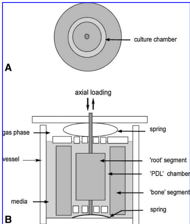
FIG. 1. Schematic drawing of the periodontal ligament (PDL) chamber, showing top (A) view and side (B) view. The model is placed in a culture vessel containing culture medium and in contact with gas phase.
