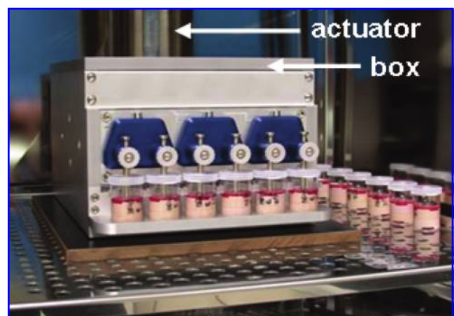
FIG. 3. PDL culture chambers ( n = 6 ) mounted in the microactuator. The actuator is computer driven and is placed in an incubator at a temperature of 37^\circ\text{C} . The cylinder on top of the box is the voice coil linear actuator. The box itself contains a hinge system, which increases the axial motion accuracy of the actuator by a factor of five and decreases the maximum amplitude of the axial motion by the same factor. Color images available online at www.liebertonline.com/ten .
