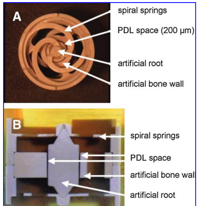
FIG. 2. Polyetherether ketone (PEEK) culture chambers for reconstruction of PDL by tissue engineering. (A) Top view of the culture chamber, showing the spiral springs holding the central, tapered cylinder representing the artificial tooth root. The circular space of 200 \mu\text{m} (PDL space) between the cylinder and the housing representing the artificial bone wall is clearly visible. (B) Longitudinal section of the same culture chamber embedded in plastic, showing the PDL space and the available volume for the culture medium. Color images available online at www.liebertonline.com/ten .
