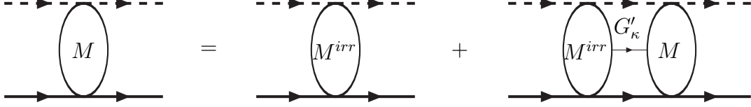
Figure 2.4: Kadyshevsky integral equation
