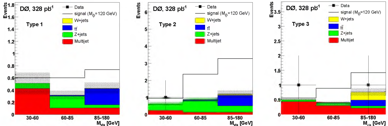
FIG. 1: Visible mass distributions for each tau type. Histograms show the signal and various backgrounds, points show the data. The error bands indicate the total uncertainty on the background estimation.
