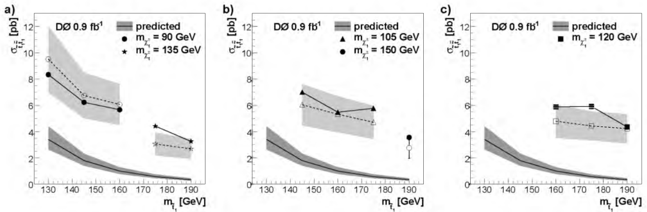
FIG. 3: Expected (open markers and dashed lines) and observed (filled markers and solid lines) Bayesian limits at 95% confidence level on the \tilde{t}_1\tilde{t}_1 cross section for all channels combined. Also shown is the \pm 1 standard deviation band on the expected limit as well as the uncertainty on the theoretical prediction caused by the choice of factorization and renormalization scales. a) For chargino masses of 90 GeV and 135 GeV, b) for chargino masses of 105 GeV and 150 GeV, c) for a chargino mass of 120 GeV.
