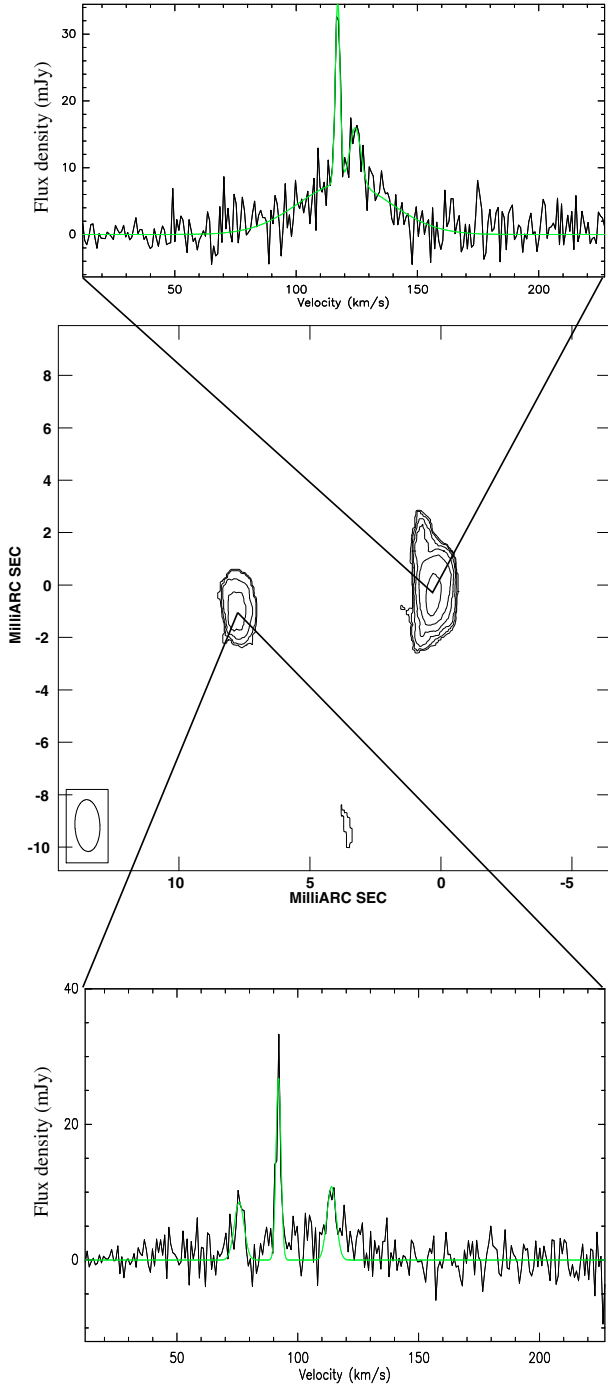
Fig. 1. Middle panel: velocity integrated water maser emission in NGC 253 from the VLBI observation on 2008 March 24 at the position of TH4. The contours start at 7 \text{ mJy km s}^{-1} and increase with factors of 2. Upper panel: spectrum of the western feature, containing one broad and two narrow components. Lower panel: spectrum of the eastern feature, containing three narrow components.
