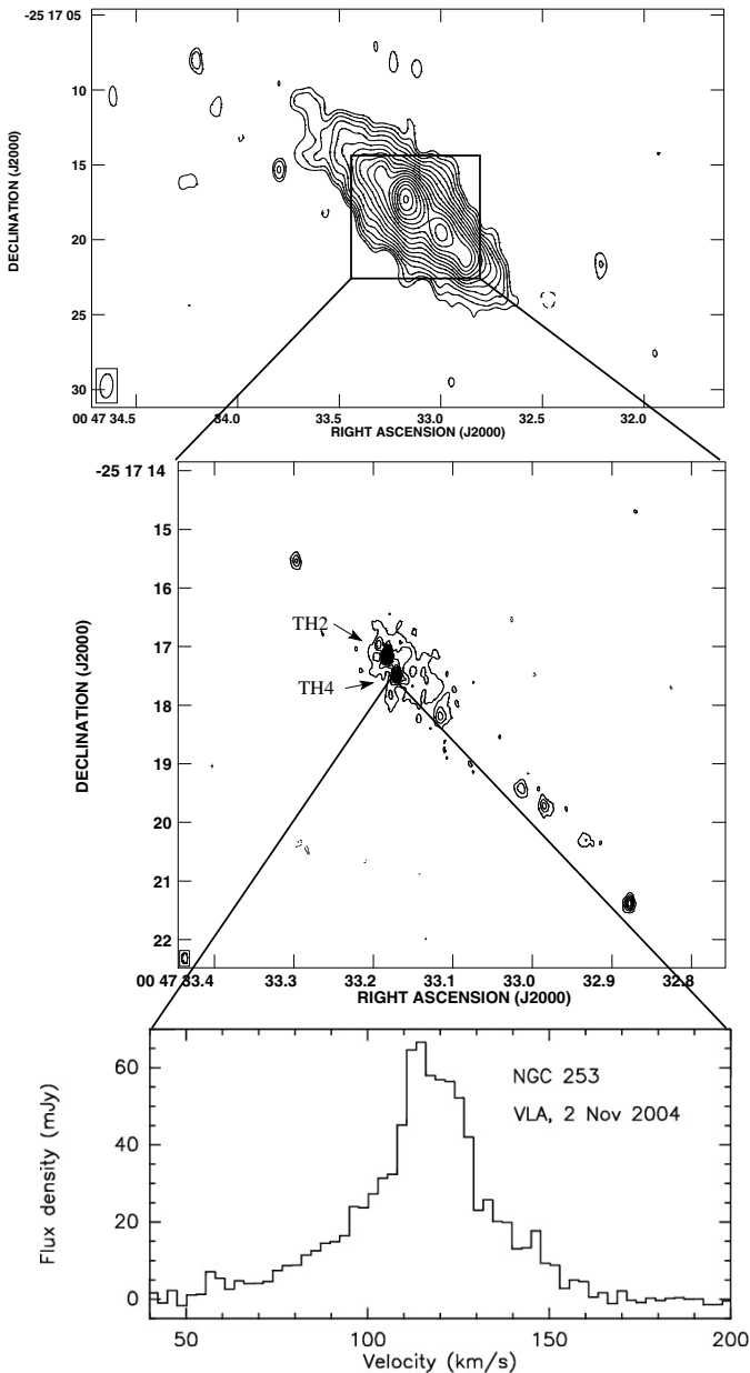
Fig. 2. Upper panel: C-array VLA image of NGC 253 at 22 GHz observed on 2008 March 24. The contours start at 0.4 mJy and increase by factors of \sqrt{2} . Middle panel: VLA A-array map of the continuum emission at 22 GHz of NGC 253 observed on 2004 November 2. The synthesized beam is shown in lower left corner . Contours are at intervals of 0.45 mJy/beam, beginning at 1.35 mJy/beam ( 3\sigma ). Lower panel: VLA A-Array spectrum of the water maser detected towards NGC 253 observed on 2004 November 2. The channel spacing is \sim 2.6 km s ^{-1} .
