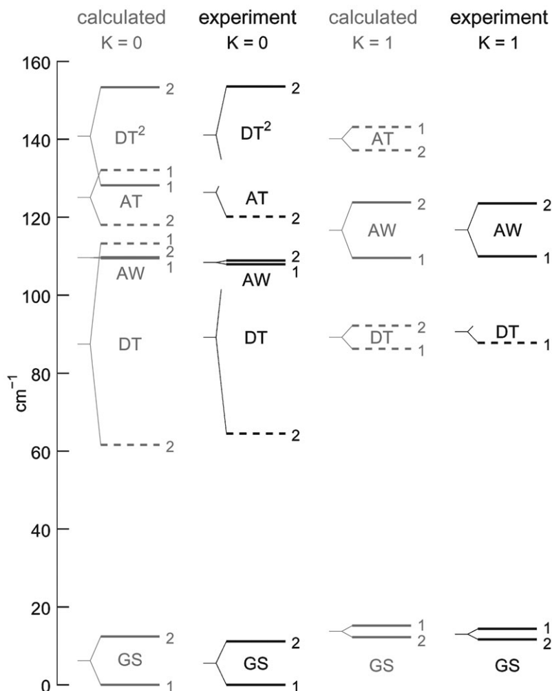
Fig. 3 VRT levels of the H 2 O dimer corresponding to the intermolecular vibrations, calculated from the CC-pol-8s potential, in comparison with experimental data. 28,38 The levels 1 and 2 are the origins, \nu_1 and \nu_2 , of the A_1 , E_1 , B_1 and A_2 , E_2 , B_2 levels, respectively. The abbreviations GS, DT, AW, and AT denote the ground state ( A' ), donor torsion ( A'' ), acceptor wag ( A' ), and acceptor twist ( A'' ) modes, following ref. 28 and 39. Solid lines refer to A' symmetry, dashed lines to A'' symmetry, with respect to the point group C_s of the equilibrium structure. Experimental levels not shown have not been measured to date.
