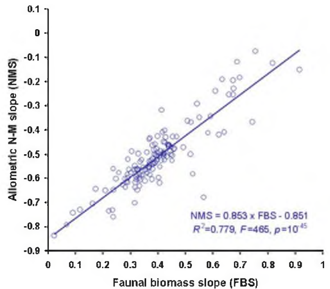
Figure 1. Linear binning and classic allometry are closely correlated. The arbitrary class interval of the \log(M) bins for our 135 real webs is 0.2 with constant linear width. In contrast to the simulation results of White et al. [43], who generated power-law distributed random numbers using inverse transformation for the Pareto distribution [8,43], the linear binning performed very well in our empirical study.
