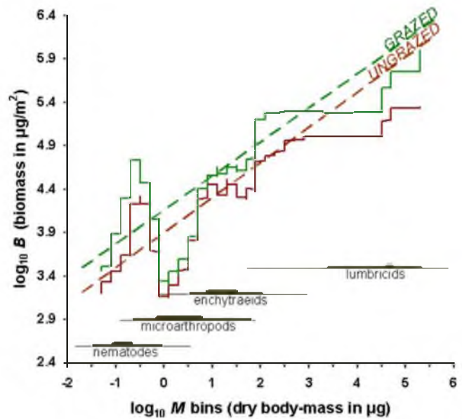
Figure 3. Repulsed frequency distribution of the faunal biomass (the aforementioned compensation between phyla is further supported by the parallel regression slopes and by the moving averages). With the chosen log( M ) interval 86% ± 22 SD of the bins between -2 and 2 (microfauna and mesofauna) and 96% ± 7.5 SD of the bins between -1.6 and 0 (microfauna) are filled. All log( M ) ranges are provided at the bottom (thin lines, min-max, medium lines, 5–95 percentile, thick lines, quartiles). doi:10.1371/journal.pone.0003573.g003
