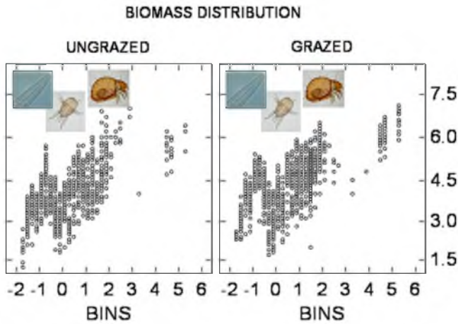
Figure 2. Distributions of log-transformed faunal biomass (ordinate) along a body size gradient (abscissa) for ungrazed and grazed agroecosystems. After lumping, grazed sites have but a higher biomass contribution of bacterial-feeding nematodes and a lower biomass contribution of hyphal-feeding enchytraeids than ungrazed sites. This structural compensation has at least two main consequences, one for the microbial consumption (microfauna grazing on bacteria, mesofauna browsing fungi) and the other for the soil aggregation and humification by larger arthropods. The peak in the biomass around 0.5 log( M ) reflects the activity of gamasid mites ( Lysigamasus , Protodinychus , Uropoda etc.) and predatory nematodes such as Aporcelaimellus . Some typical genera are shown: from left to right, Chiloplacus , a bacterial-feeding nematode highly tolerant for grazing pressure and land-use intensity, the predatory mite Alliphis and the microphytophagous Rhysotritia [10]. doi:10.1371/journal.pone.0003573.g002
