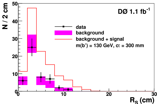
FIG. 2: Observed R_S distribution for di-EM pairs with mass greater than 75 GeV (black points), expected distribution from prompt sources with its uncertainty (shaded rectangles) and the expected distribution in presence of b' quark with mass of 130 GeV and lifetime c\tau = 300 mm (solid line).
