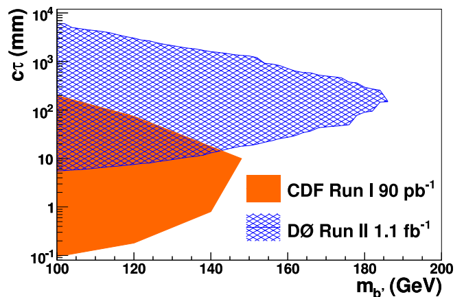
FIG. 4: 95% C.L. exclusion region of b' lifetime ( c\tau ) vs. mass for CDF Run I [4] and current DØ result.
