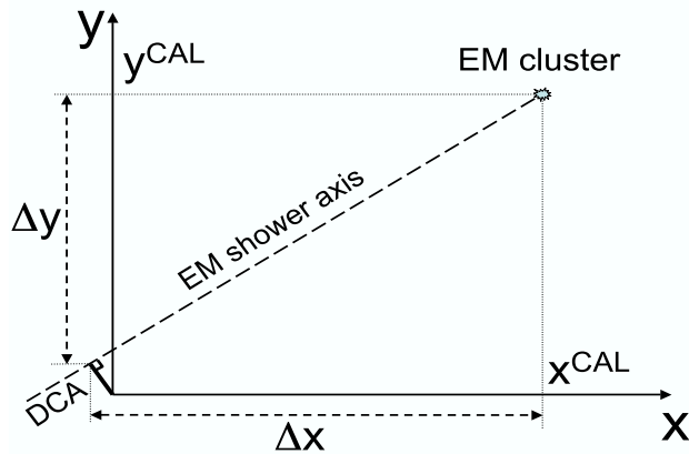
FIG. 1: Definition of the reconstructed EM particle trajectory. In the D0 coordinate system the equation of the trajectory is given by \Delta x \cdot (y - y^{CAL}) = \Delta y \cdot (x - x^{CAL}) . The distance from the beam line to the EM shower maximum \sqrt{(x^{CAL})^2 + (y^{CAL})^2} is typically around 90 cm.
