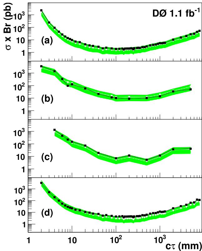
FIG. 3: Expected (white triangles) and observed (black squares) 95% C.L. upper limits on the cross section of a long-lived particle times the branching fraction of its decay to either a pair of electrons or photons for (a) \cancel{E}_T > 30 GeV and M > 20 GeV, (b) 20 < M < 40 GeV, (c) 40 < M < 75 GeV, and (d) M > 75 GeV. All observed upper limits are within one standard deviation (shaded band) from the expected limits.
