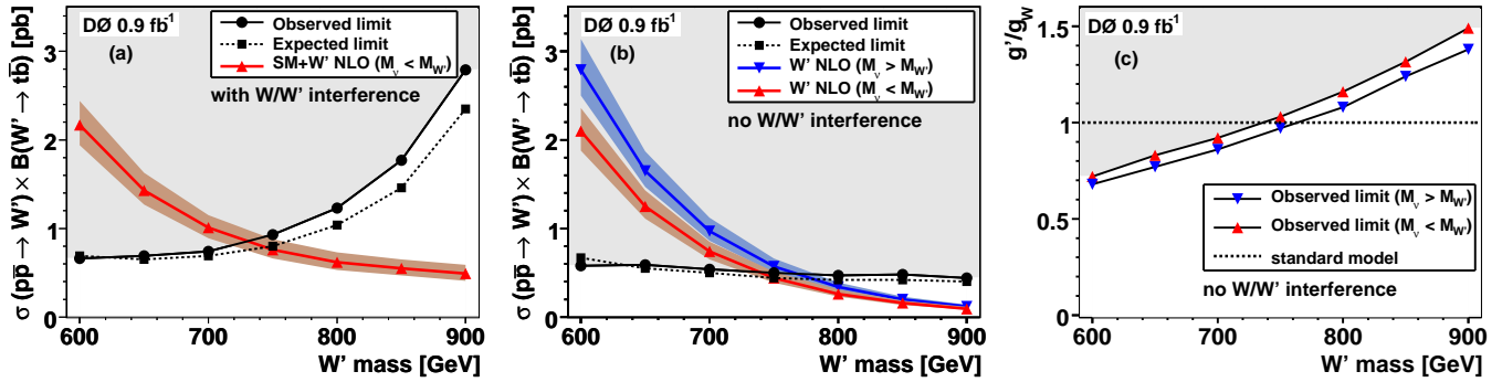
FIG. 2: NLO theory cross sections and 95% C.L. limits for \sigma_{W'} \times \text{B}(W' \rightarrow \text{tb}) as a function of W' mass for (a) W'_L production and (b) W'_R production. Observed limits on the ratio of coupling constants g'/g_w are shown in (c). The shaded regions are excluded by this analysis.
