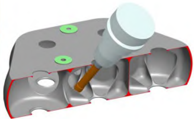
Figure 4. Balance Arm using the ASTRON extreme light-weighting technique. Large internal volumes (pockets) are created by milling through small entrance holes. The weight of the 540 x 400 x 57 mm aluminium balance arm is 2kg, which corresponds to lightweighting percentage of 90%. Internal ribs in the pockets improve the overall stiffness.
