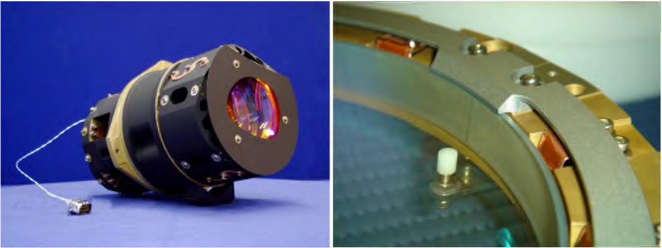
Figure 9. The Camera consists of 2 ZnSe aspheres and 1 CaF2 asphere (Left image). All lenses are mounted using CTE compensation mechanisms in order to maintain accurate alignment at both room temperature and operating temperature. Copper spring pads plated with indium are used for a fast cool down and warm up and are clearly visible in the detail of the corrector lens mount in the right image.
