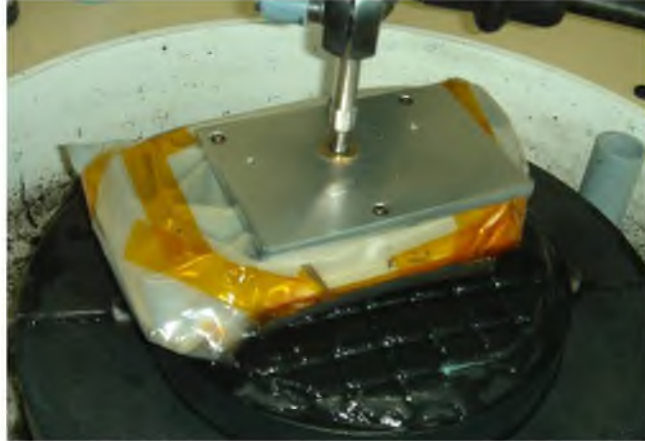
Figure 3. In a newly developed technique the bare aluminium mirror is conventionally polished to optical quality, The mirror is wrapped in plastic to avoid contamination during polishing. Achieved surface figures are <math><200\text{nm}</math> together with a surface roughness in the order of 1nm.
