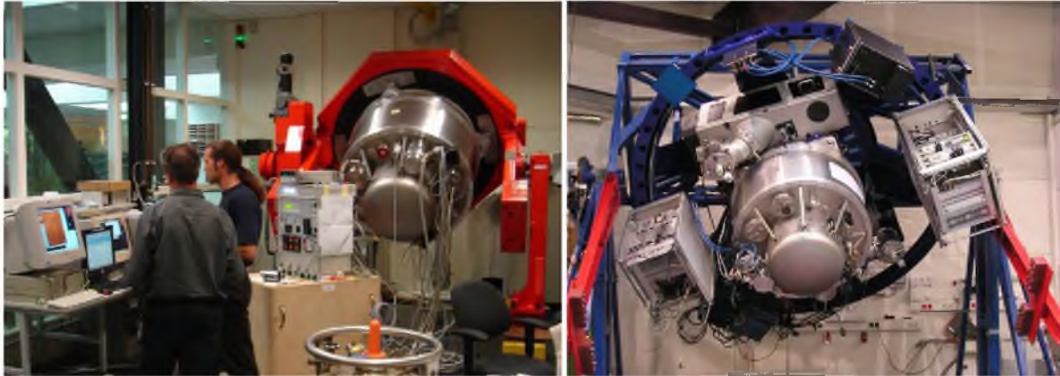
Figure 13. X-shooter near infrared spectrograph during tests at NOVA-ASTRON (left image). The cryostat is mounted on a dummy backbone that is mounted on the telescope simulator (right). The Cold Optical Box is located inside the cryostat. Other equipment comprise the cryogenic control electronics (center) and 3 workstations to control the detector, run the VLT software and analyze all data. The top of one of six liquid nitrogen tanks is visible in the front. X-shooter integrated with the backbone, UVB and VIS spectrographs and electronics in the ESO lab (right image).
