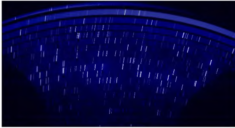
Figure 15. X-shooter NIR Th-Ar spectrum at preliminary acceptance Europe.
