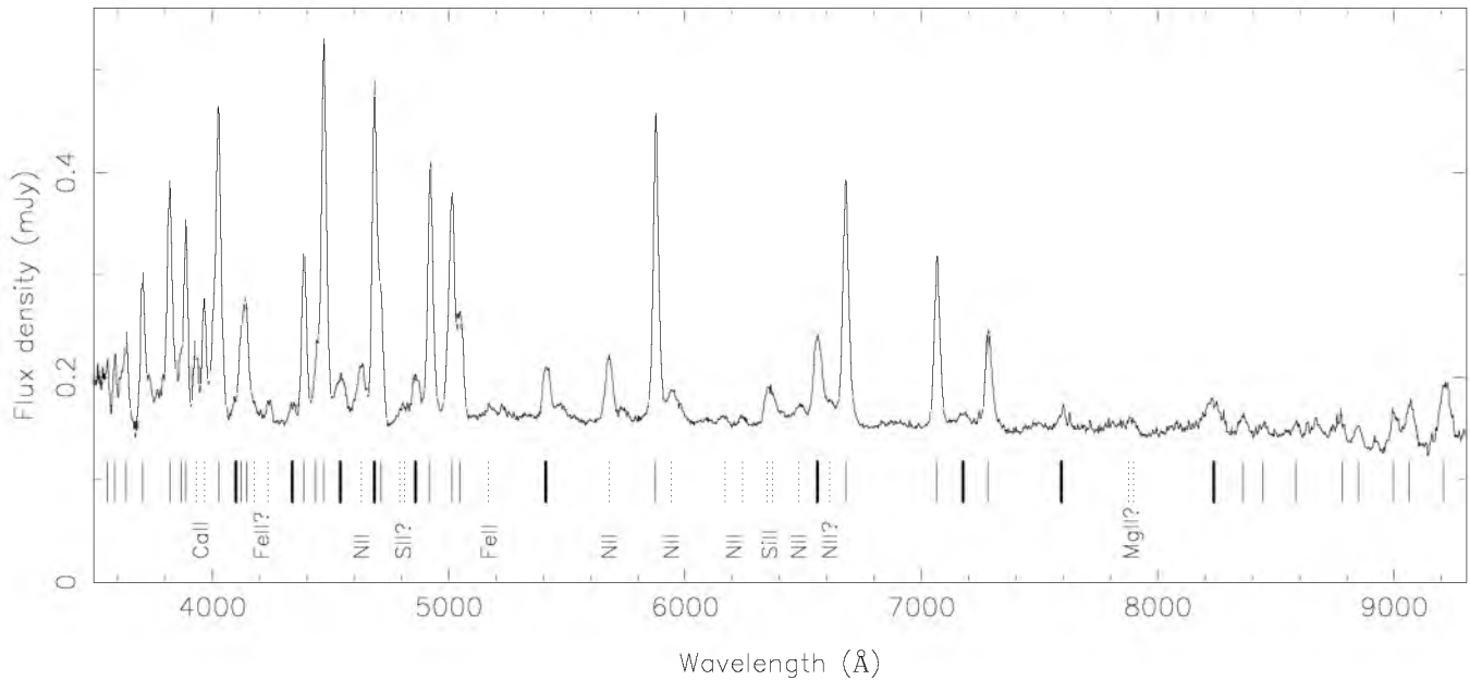
Figure 4. Average spectrum of SDSS J0804+1616. Thin and thick solid lines indicate neutral and ionised helium lines, respectively, while dotted lines indicate metal lines as labelled. See Figure 5 for a detailed view of the shapes of the emission lines.
