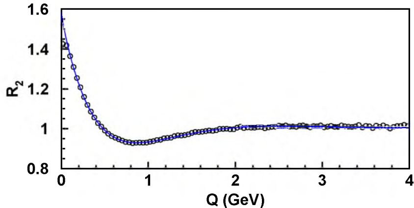
Figure 1: The Bose-Einstein correlation function R_2 for events generated by PYTHIA. The curve corresponds to a fit of the one-sided Lévy parametrization, Eq. (13).
