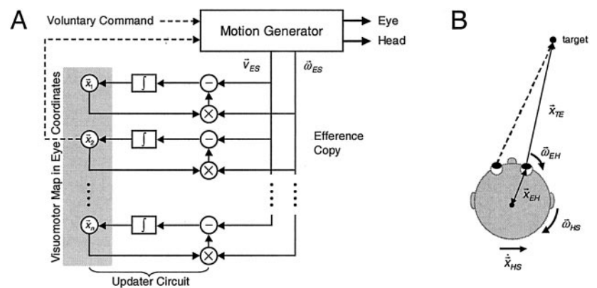
Figure 7. Retinotopic remapping. A , A target is selected from an eye-centered target map ( \tilde{x}_1, \tilde{x}_2, \dots, \tilde{x}_n ), and its retinal error is passed to a motion generator that can rotate the eyes and head as well as translate the head. The motion generator can also be driven using voluntary commands. In generating the motion, it provides feedback signals about eye and head motion, as given by \tilde{\omega}_{ES} (the rotary velocity of the eyes in space, \tilde{\omega}_{ES} = \tilde{\omega}_{HS} + \tilde{\omega}_{EH} ) and \tilde{v}_{ES} (the translational velocity of the eyes, \tilde{v}_{ES} = \tilde{\omega}_{HS} \times \tilde{x}_{HS} , with \times indicating the vector cross-product). Both signals, computed in eye coordinates, are used to update the retinotopic target map. Updating circuits use local information about target depth and direction (as stored in the target map) to determine how that same representation is remapped during the motion. B , The derivation of the updating equation (Eq. 3). If the eyes are rotating, the target moves in opposite direction relative to the eyes, according to \dot{\tilde{x}}_{TE} = \tilde{x}_{TE} \times \tilde{\omega}_{ES} . Likewise, when the eyes are translating, the target moves with opposite velocity relative to the eyes, as given by \dot{\tilde{x}}_{TE} = -\tilde{v}_{ES} = \tilde{x}_{EH} \times \tilde{\omega}_{HS} - \dot{\tilde{x}}_{HS} . Combining the two equations yields Equation 3.
