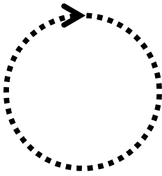
Figure 2: A prototypical round path
