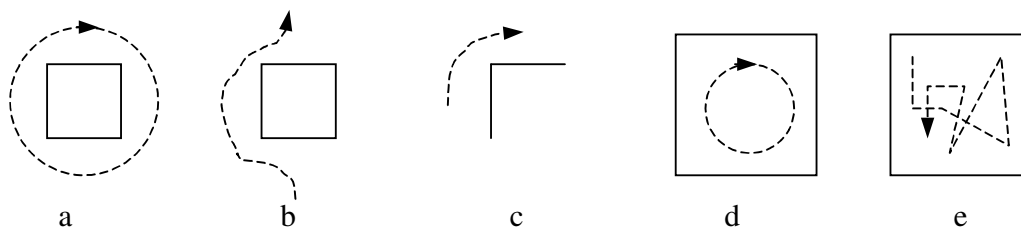
Figure 1: Paths corresponding to the preposition round
