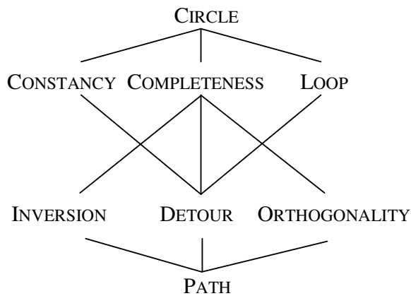
Figure 3: Strength of round properties
