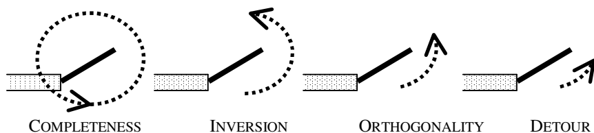
Figure 4: Four of the possible interpretations of round the door
