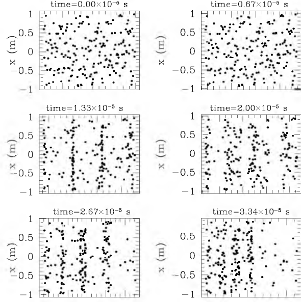
Fig. 3a. Run 1: (z,x) -behaviour of the particles during their passage in the cavity (from left to right; from top to bottom). On the horizontal axis is plotted the z -coordinate of all particles, subsequently for z = 2, 4, 6, 8 and 10 km. Except for t = 3.34 \cdot 10^{-5} s, the horizontal spacing between the long ticks is 0.02 m (e.g. \Delta z \approx 0.08 m for t = 0 s). In the last plot, the spacing between the long ticks is 0.05 m. Bunching clearly occurs at t = 1.33 \cdot 10^{-5} s, ‘de-bunching’ at t = 2.0 \cdot 10^{-5} s and ‘re-bunching’ at t = 2.67 \cdot 10^{-5} s.
