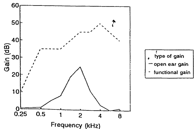
Figure 4. Functional gain (FG) and open ear canal gain as a function of frequency obtained in patient V6.
