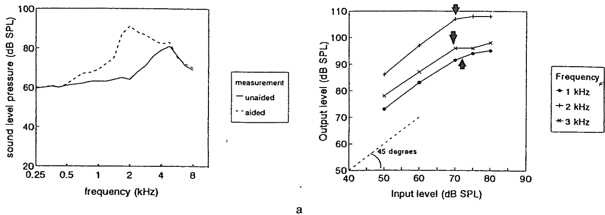
Figure 8. Typical examples of input-output curves constructed from the open ear recordings of patient V8 (Figure 8a) and O5 (Figure 8b) at 1, 2, and 3 kHz. The arrows indicate the input level at which output started to level off.
