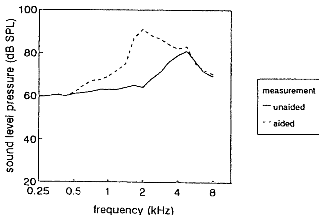
Figure 1. Typical example of aided and unaided sound pressure levels measured in the open ear canal as a function of frequency (patient V6). The frequency sweep used was presented at a level of 60 dB SPL.
