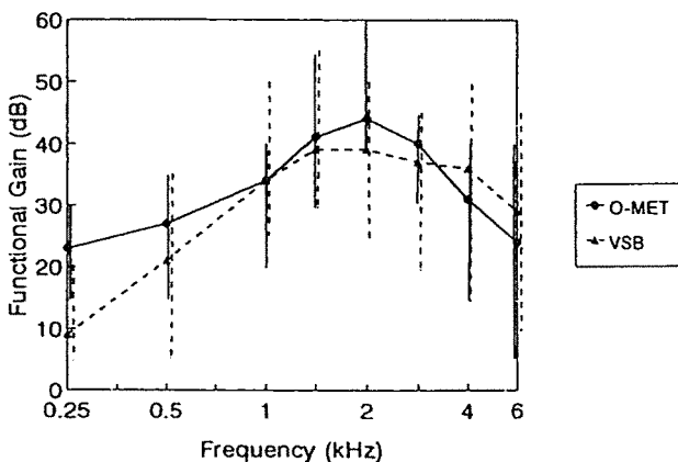
Figure 2. Mean functional gain (and range) as a function of frequency of the VSB users and Otologics MET users. The full vertical lines indicate the range of the Otologics MET data and the broken vertical lines that of the VSB data.
