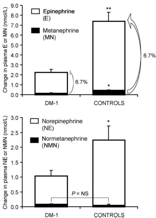
FIG. 1. Mean ( \pm SEM) increases in plasma epinephrine and metanephrine ( top ) and in plasma norepinephrine and normetanephrine ( bottom ) in response to hypoglycemia. In both patients and controls, the increase in plasma metanephrine was 6.7% that of plasma epinephrine ( P = NS). *, P < 0.05; **, P < 0.001 (higher plasma concentration vs. that in diabetic patients).
