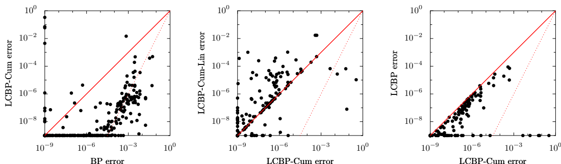
Figure 6: Pairwise comparisons of errors of various methods for the same instances as in Figure 3. Only the cases have been plotted for which both approximate inference methods converged.
