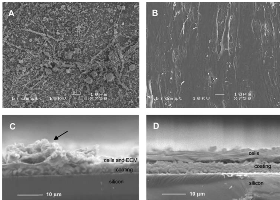
FIG. 7. Scanning electron micrographs of osteoblast-like cells cultured for 16 days. (A) Substrate without TGF- \beta 1. Note the formation of a mineralized extracellular matrix. (B) Substrate with 10 ng of TGF- \beta 1. Note that mineralization has not occurred. (C, D) Cross-sections of the samples shown in A and B , respectively. Visible are the silicon substrate, coating, and cell layer. In C , mineralized matrix is visible (arrow). In D , a thick confluent cell layer is present.
