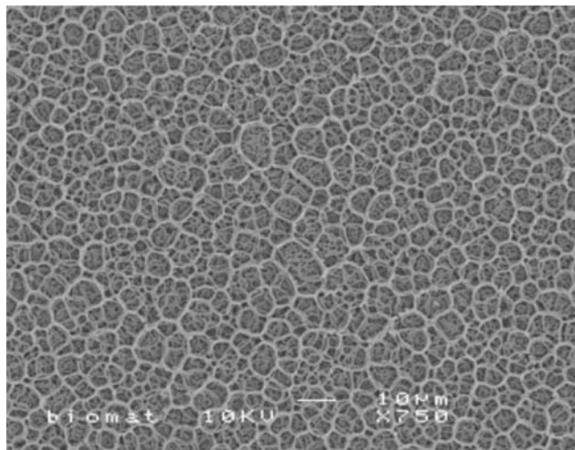
FIG. 1. Scanning electron micrograph of the porous CaP coating before cell culture.
