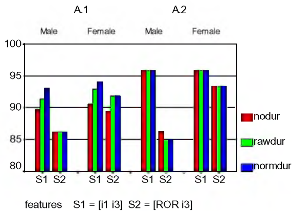
Figure 1: Correct classification in %, left = exp. A.1, right = exp. A.2.
