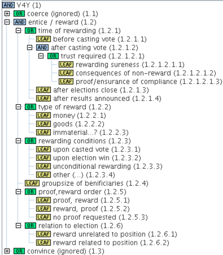
Fig. 1. Attack tree for vote buying
