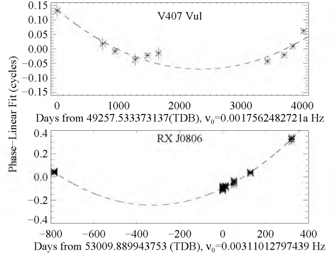
Figure A1. Phase residuals of V407 Vul (top panel) and HM Cnc (bottom panel) after subtraction of constant frequency models. The dashed line shows our parabola ephemeris subtracted the linear fit.
