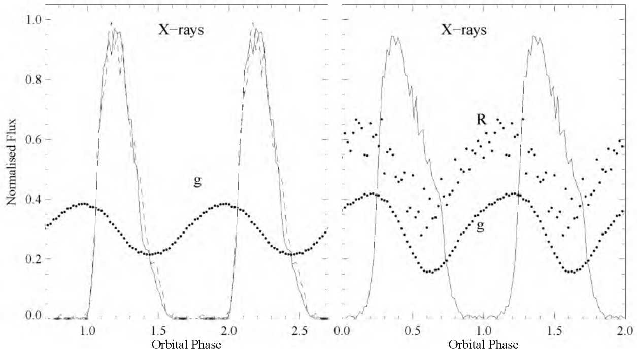
Figure 5. X-Ray/optical phase folded light curve of V407 Vul (left) and HM Cnc (right) using the ephemeris of Table A1 and (Strohmayr 2005) respectively. For the X-ray light curves of V407 Vul we re-analysed Chandra observations, with the solid line showing data from 19 th February 2003 and the dashed line from 24 th November 2003. For HM Cnc, the X-rays were adapted from Strohmayr (2005). We overplot the optical g' band showing our results. For HM Cnc we also show the VLT/FORS data (Israel et al. 2002) taken in the R filter (top).
