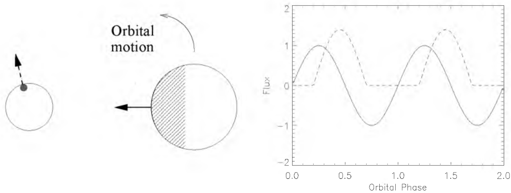
Figure 7. In the left-hand panel we show a schematic picture of the primary star (left) with an X-ray emitting spot which has a peak of X-ray emission in the direction indicated by the dashed arrow. The relative sizes of the two stars are drawn to match masses of M_1 = 0.53 M_\odot and M_2 = 0.12 M_\odot (see text). The secondary star, which orbits counter-clockwise, has a heated face (shaded) whose peak emission is in the direction of the solid arrow. The figure is arranged to give the optical (solid) and X-ray (dashed) light curves shown on the right, which have the same relative phasing as both V407 Vul and HM Cnc.
