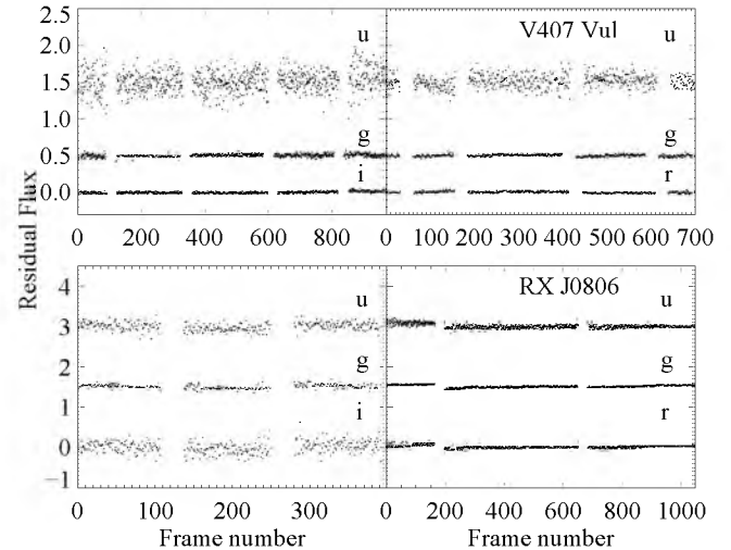
Figure 6. V407 Vul (top panel) and HM Cnc (bottom panel) light curves after removal of the sinusoidal pulsations. For each object the data from the first observing period is in the left and the second in the right. There are no significant variations of either source. We inserted gaps between different nights.
