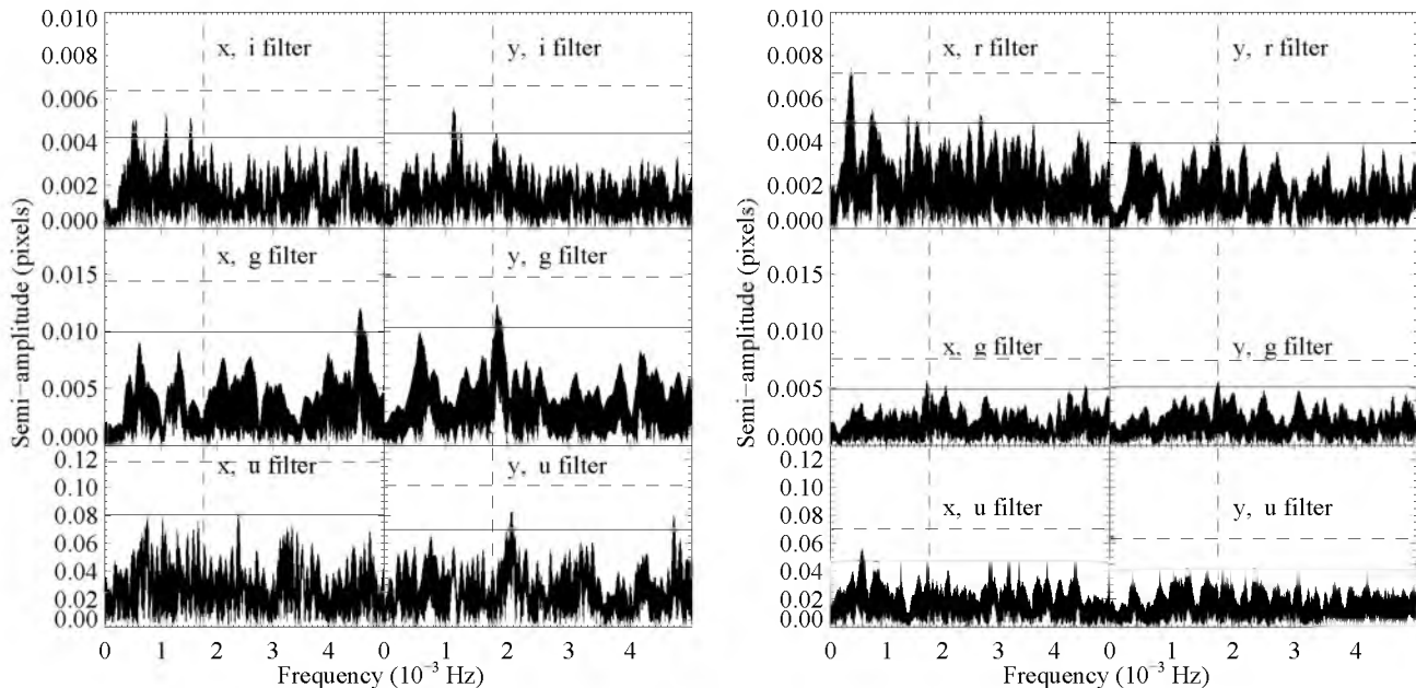
Figure 2. Each panel shows the amplitude spectra of the x (left) and y (right) variation of the position of V407 Vul for the three filters i' or r' , g' , and u' from top to bottom. The left panel shows the May 2003 data while the right shows the August 2005 data. The vertical dashed lines show the position of the 569 sec period. The solid horizontal lines show the 99.9 percent significance level for a known period and the dashed horizontal lines show the same level for an arbitrary period.
