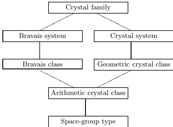
Figure 1: Hierarchy of classification
