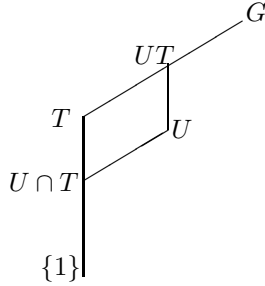
Figure 2: A subgroup U of the space group G
