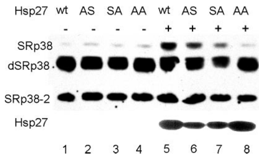
Figure 5. Effect of the phosphorylation state of Hsp27 on rephosphorylation of SRp38 after heat shock. T-REx HeLa cell lines expressing different mutants mimicking partially unphosphorylated Hsp27 were cultured with (+ Hsp27 or its mutants) or without (- Hsp27 or its mutants) doxycycline, heat shocked, and harvested 6 h after recovery at 37°C. Lanes 1 and 5: Hsp27 wild-type (Wt) cell line; lanes 2 and 6: Hsp27 S15A (AS) cell line; lanes 3 and 7: Hsp27 S90A (SA) cell line; lanes 4 and 8: Hsp27 S15/90A (AA) cell line. SRp38 indicates the fully phosphorylated form, dSRp38 the (partially) dephosphorylated form, whereas the bottom panel shows the alternative spliced form of SRp38 (SRp38-2). The bottom panel shows the induced expression level of wild-type or mutant hamster Hsp27.
