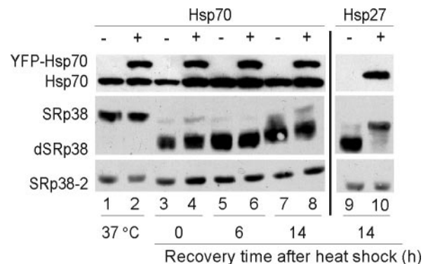
Figure 7. Overexpression of Hsp70 does not enhance SRp38 rephosphorylation after heat shock. Western blot showing Hsp70 levels and the different forms of SRp38 found after heat shock and recovery in the presence or absence of exogenous Hsp70. HEK-293 cells expressing YFP-Hsp70 were cultured with (+) or without (–) doxycycline, and either heat shocked and harvested at the indicated time points (lanes 3–8) or cultured at 37°C (lanes 1 and 2). The top panel shows the staining for the induced Hsp70 (YFP-Hsp70) and the endogenous Hsp70 (Hsp70). SRp38 indicates the fully phosphorylated form and dSRp38 the (partially) dephosphorylated form. For comparison the Western blots showing Hsp27 levels and the different forms of SRp38 found in HEK-293 cells after heat shock and 14 h of recovery in the absence or presence of exogenous Hsp27 are also shown (lanes 9 and 10).
