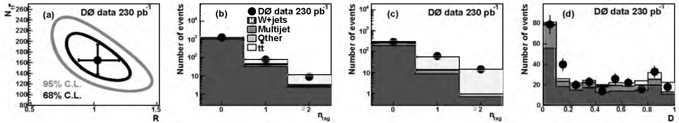
FIG. 1: (a) The 68% and 95% statistical confidence contours in the (R, N_{tt}) plane. The point indicates the best fit to data. Observed number of events and fitted sample composition in the 0, 1, and 2-tag samples (b) in the \ell + 3 jets sample and (c) in the \ell + \geq 4 jets sample. (d) Observed and fitted distribution of the discriminant \mathcal{D} .
