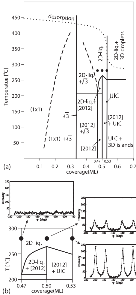
FIG. 1. (a) Phase diagram of a Bi monolayer on Cu(111). The nomenclature is explained in the text. The dotted line indicates the temperature above which desorption is too rapid to perform our type of experiments. (b) A detailed view of the phase diagram around 0.5 ML Bi and 250 °C, together with background-subtracted azimuthal scans through the diffuse scattering rings at Bi coverages of 0.47, 0.50, and 0.53 ML and at a temperature of 280 °C. The solid circles in the phase diagrams indicate the conditions for the azimuthal scans.
