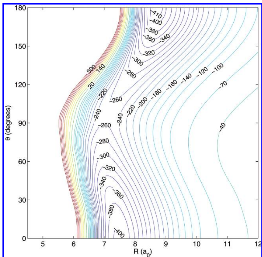
Figure 5. Lowest spin-orbit adiabatic potential energy surface. Energy (in \text{cm}^{-1} ) relative to the \text{Br}(^2P_{3/2}) and \text{HCN} ground states.
