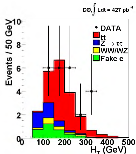
FIG. 1: H_T distributions in the e\mu channel for expected signal (assuming m_t = 175 GeV and \sigma_{t\bar{t}} = 7 pb), expected background, and data after both lepton and jet requirements (corresponding to the second line of Table IV).
