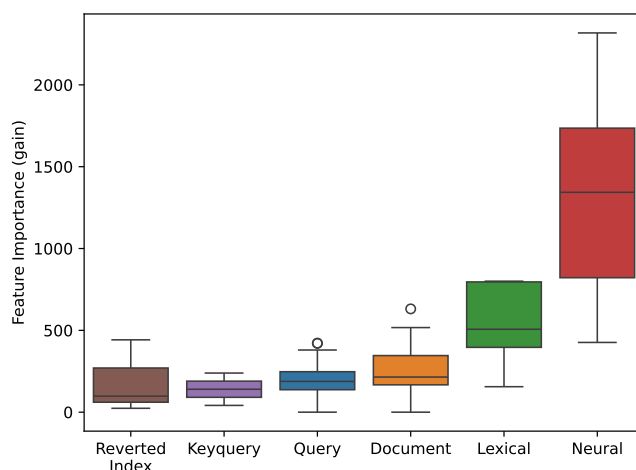
Figure 1: Feature importance per feature type. For feature importance, we use the ‘gain’ metric, which measures, per feature, the total performance gain obtained from splits using that feature.
