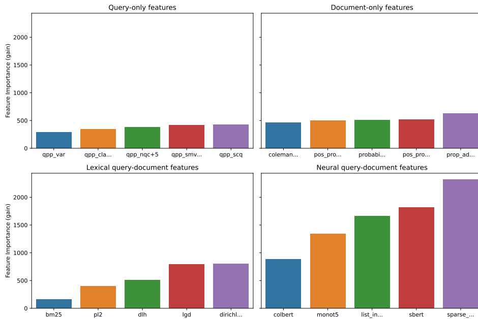
Figure 2: Top 5 most important features for query-only, document-only, and query-document (lexical and neural matching scores) features. For feature importance, we use the ‘gain’ metric, which measures, per feature, the total performance gain obtained from splits using that feature.
