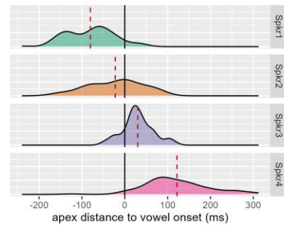
Figure 2: Distribution of distance of apex to vowel onset by speaker. Solid line represents vowel onset.
