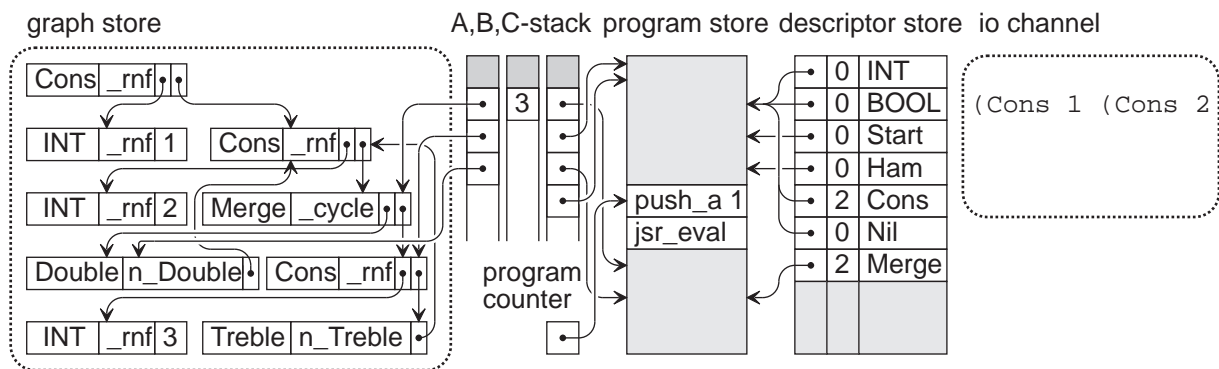
Figure 3. The ABC-machine.
