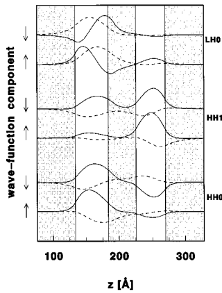
FIG. 5. Envelope function of wave-function components at k=2.6 \times 10^8 \text{ m}^{-1} in the \langle z \rangle direction for the 59.4–33.9–42.4 Å ADQW with a density of 1.5 \times 10^{16} \text{ m}^{-2} . Solid lines, HH component; dashed lines, LH component.
