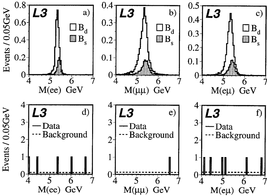
Fig. 1. Predictions for the dilepton invariant mass distributions for a) B^0 \rightarrow e^+e^- , b) B^0 \rightarrow \mu^+\mu^- , and c) B^0 \rightarrow e^\pm\mu^\mp decays, assuming the integrated luminosity and efficiencies of this analysis and a nominal branching fraction of \text{Br}(B^0 \rightarrow \ell^+\ell^-) = 10^{-5} for each process. Mass spectra obtained from the data (solid line) for d) e^+e^- , e) \mu^+\mu^- , and f) e^\pm\mu^\mp ; the dashed lines show the background predicted by Monte Carlo.
