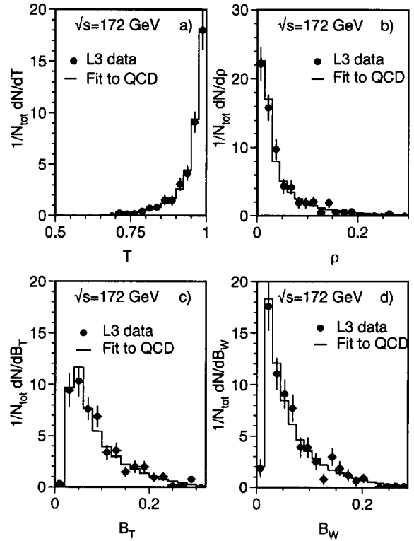
Fig. 7. Measured distributions of thrust, T , scaled heavy jet mass, \rho , total, B_T , and wide, B_W , jet broadening in comparison with QCD predictions at 172 GeV. The experimental errors include statistical and systematic uncertainties.
