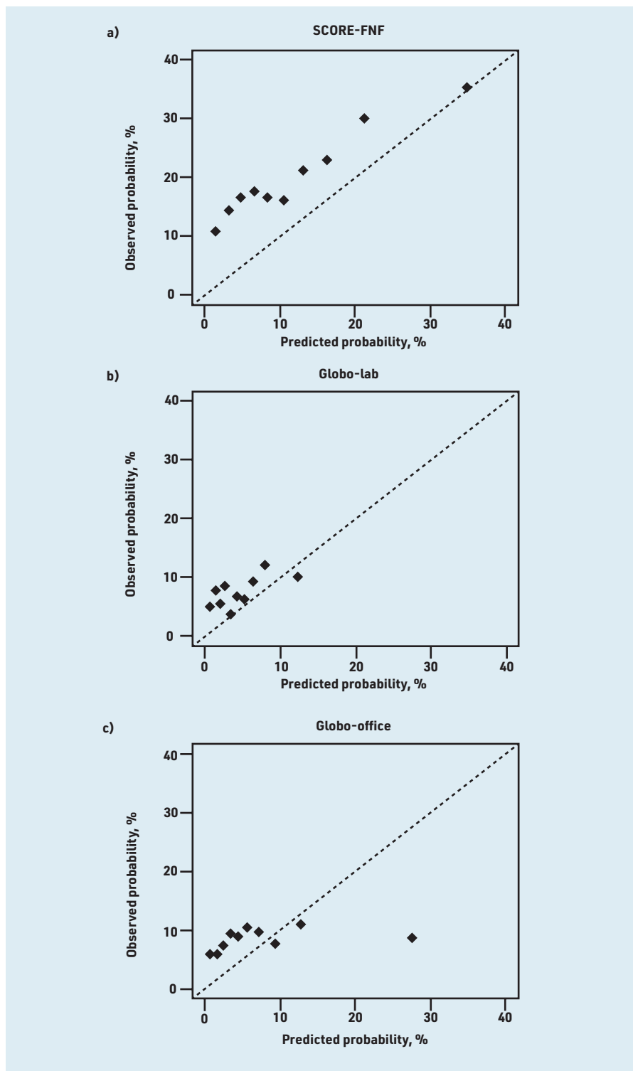
Figure 2. Calibration plots of predicted versus observed risks of a) SCORE-FNF; b) Globo-lab; and c) Globo-office. Patients were grouped based on deciles of predicted risk. The diagonal line represents the line of perfect calibration. See Supplementary Table S7 for more details. Globo-lab = Globorisk-laboratory. Globo-office = Globorisk-office. SCORE-FNF = SCORE fatal and non-fatal.
