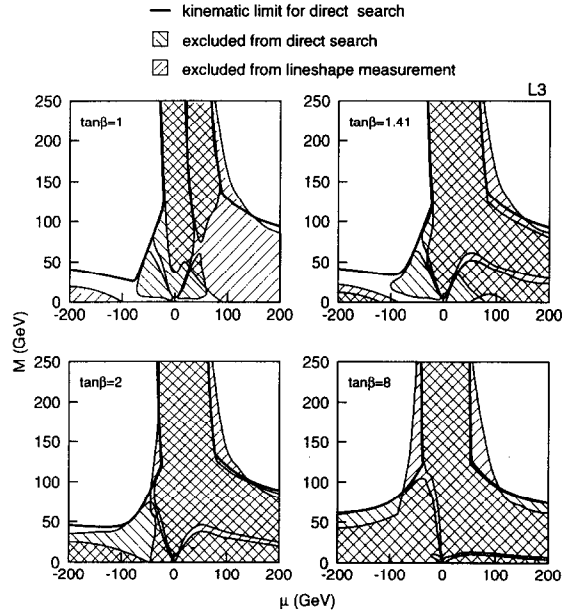
Fig. 5. The excluded regions of the MSSM parameter space at the 95% C.L. as a function of the parameters M and \mu . The kinematical limit corresponds to the sum of the lightest and next to lightest neutralino masses being equal to the center-of-mass energy. The exclusion coming from the lineshape measurement goes beyond the kinematic limit of the direct search.
