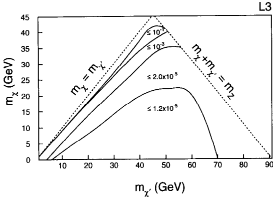
Fig. 3. Contour plot of the 95% C.L. upper limits on \text{Br}(Z \rightarrow \chi\chi') versus the \chi and \chi' masses. The solid lines separate the regions, where the limit on the branching ratio is smaller than the value shown, while the dashed lines show the kinematical limits of the channel.
