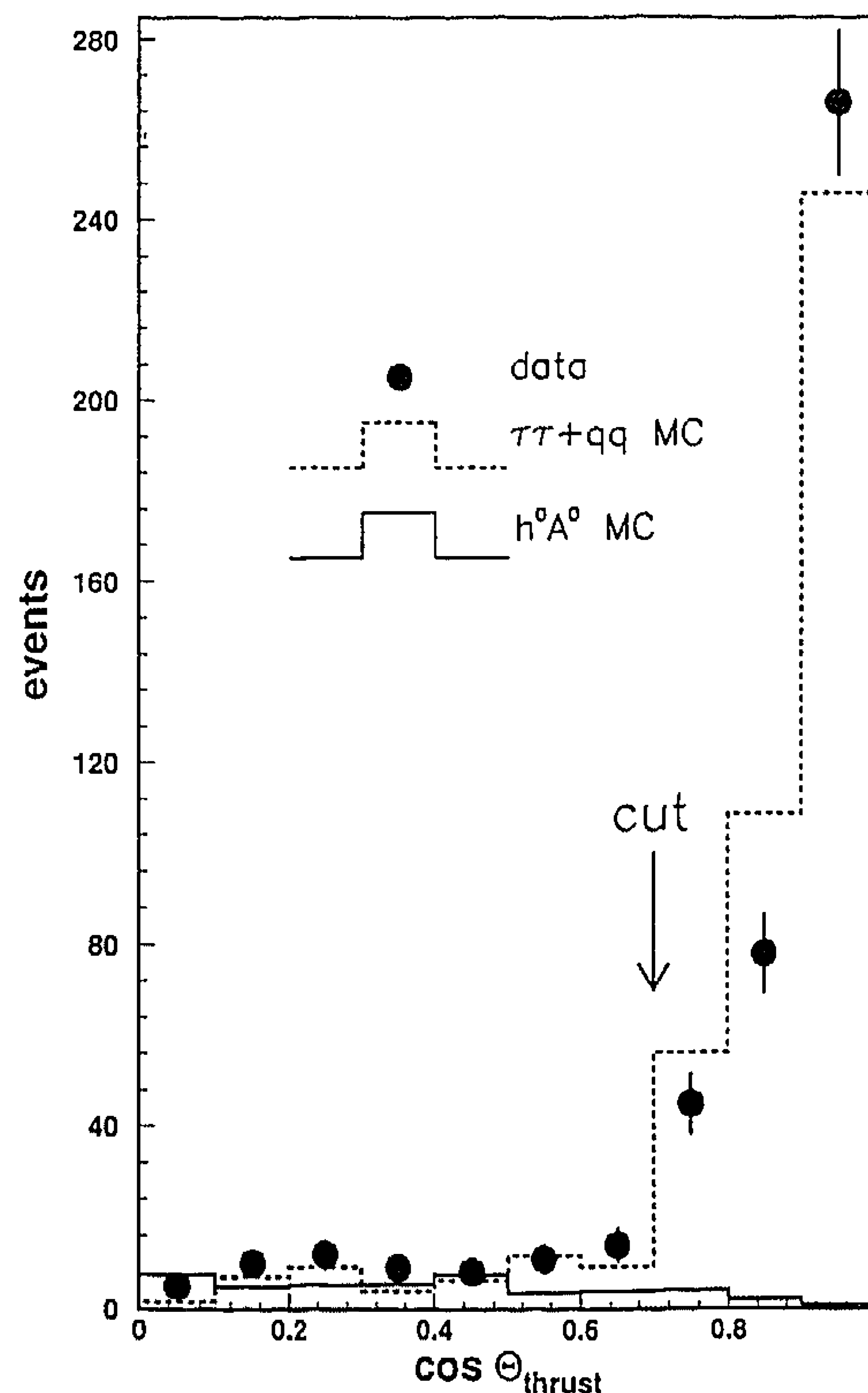
Fig. 4. \cos \theta_{\text{thrust}} for data, q\bar{q} simulation and signal simulation in the h^0 A^0 \rightarrow \tau\bar{\tau}b\bar{b} search. The peak in the data and in the q\bar{q} simulation is due to the E_{\text{vis}} < 80 GeV cut, which enhances the rate of events losing energy along the beam direction. Less than eight clusters in the tau hemisphere leading to exactly two jets is required.
