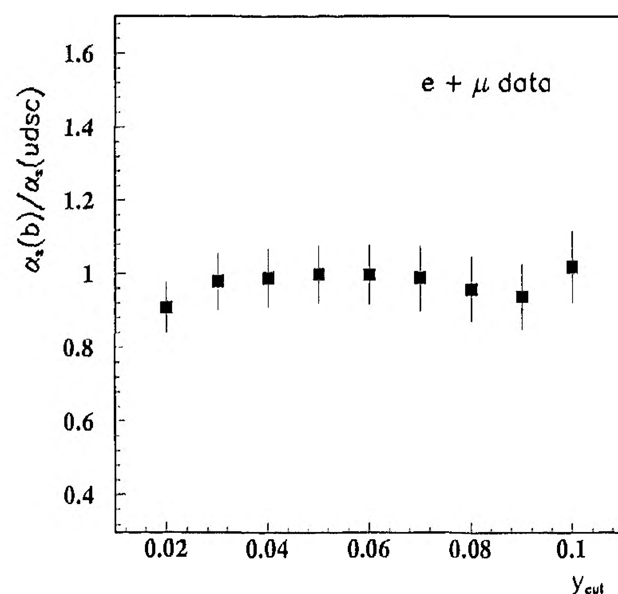
Fig. 1. Measured \alpha_s(\text{b})/\alpha_s(\text{udsc}) ratios, for the inclusive lepton sample (muons and electrons), as a function of the jet resolution parameter y_{\text{cut}} . The error includes the statistical and the systematic contributions.
