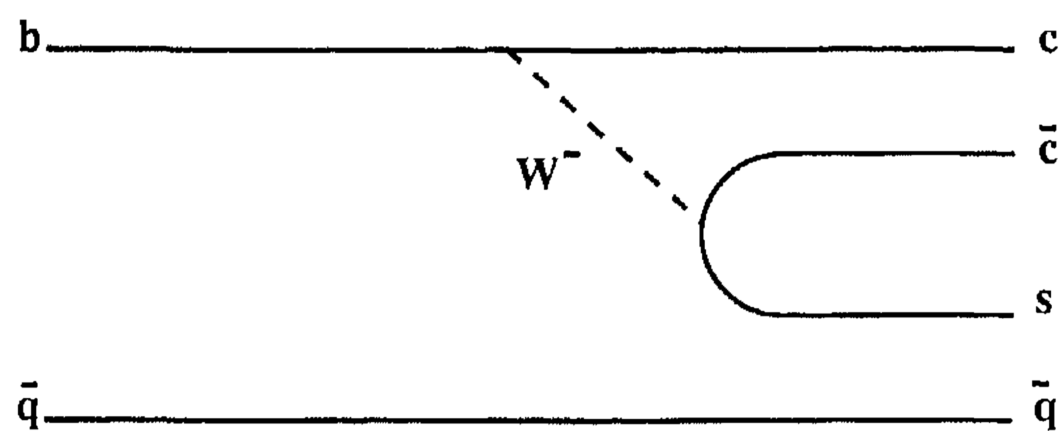
Fig. 1. Diagram for b(\bar{b}) \rightarrow [c\bar{c}] + X .
