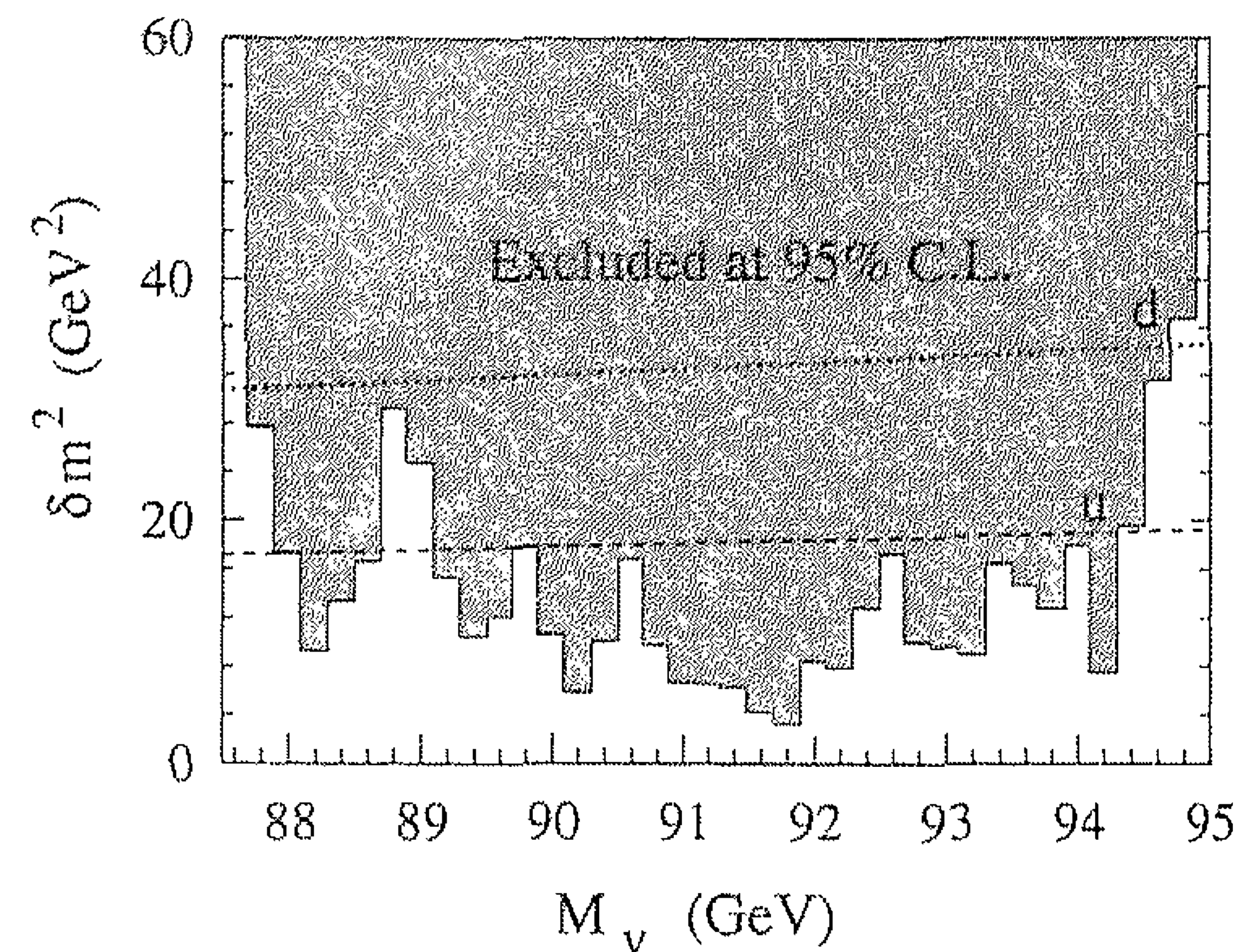
Fig. 3. Limits on the mixing parameter \delta m^2 as a function of the resonance mass. We exclude, at the 95% CL, values of \delta m^2 above the histogram (shaded region). The value of \delta m^2 expected from a potential model is plotted for quarkonia of d-type (dotted line) and u-type (dashed line) quarks. Resonances whose mixing with the Z is larger than the limits shown on \delta m^2 are excluded by this search.
